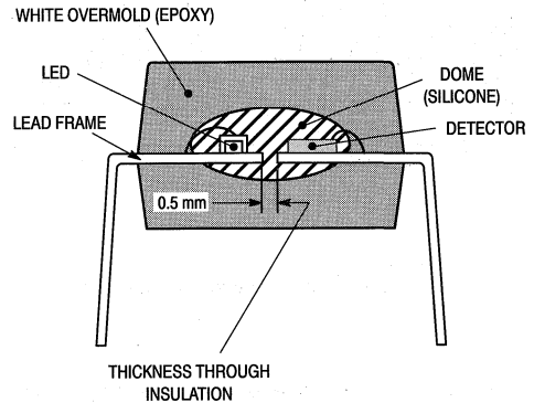
Figure 5. Geometric Design for Optoisolators
