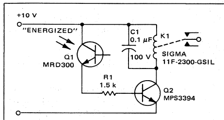
FIGURE 25 – Light-Operated Relay
