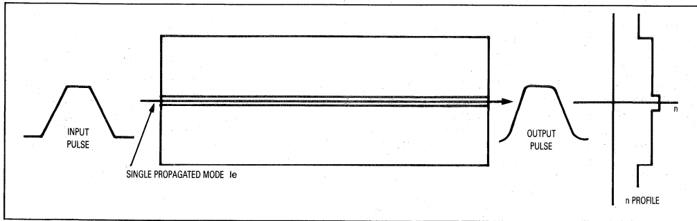
Figure 17. Propagation Along A Single Mode Step Index Fiber
