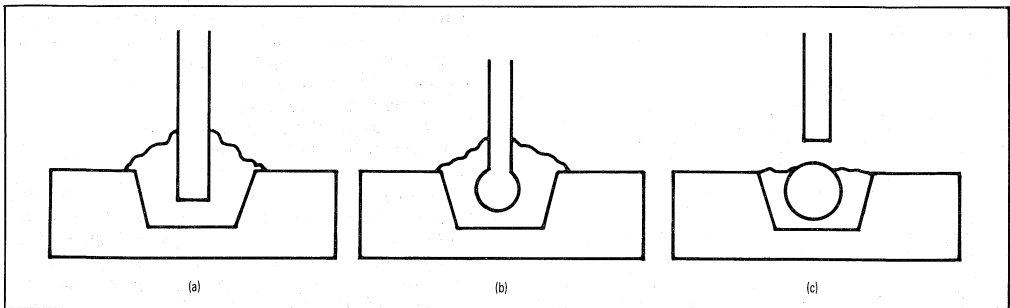
Figure 25. Fiber Coupling To A Burrus Diode:
