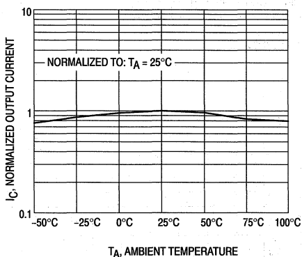
Figure 1. Output Current versus Ambient Temperature
