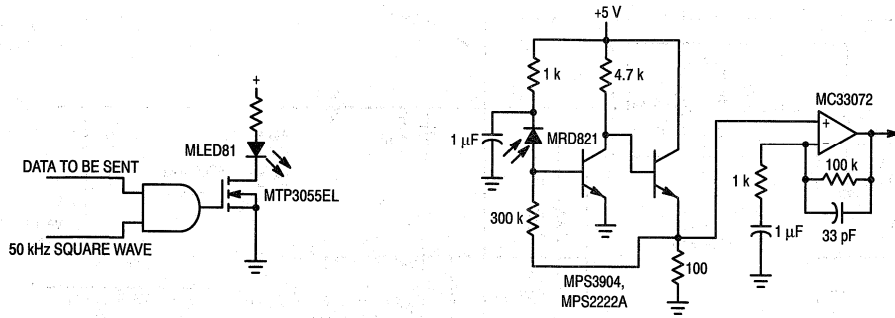
Simple Discrete Front End with Op Amp
