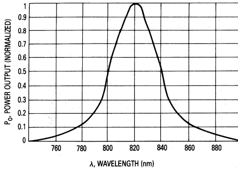
Figure 3. Typical Spectral Output versus Wavelength
