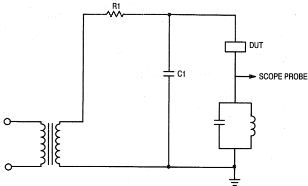
Figure 3. Narrowband Partial Discharge Test Circuit
