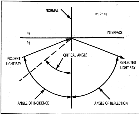
Figure 5. Light Incident At Greater Than Critical Angle
