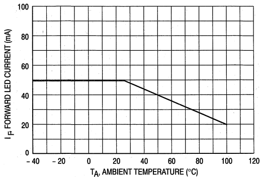
Figure 1. Maximum Allowable Forward LED Current versus Ambient Temperature
