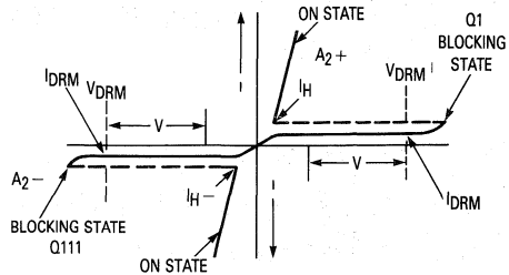
Figure 3. Triac Voltage-Current Characteristic
