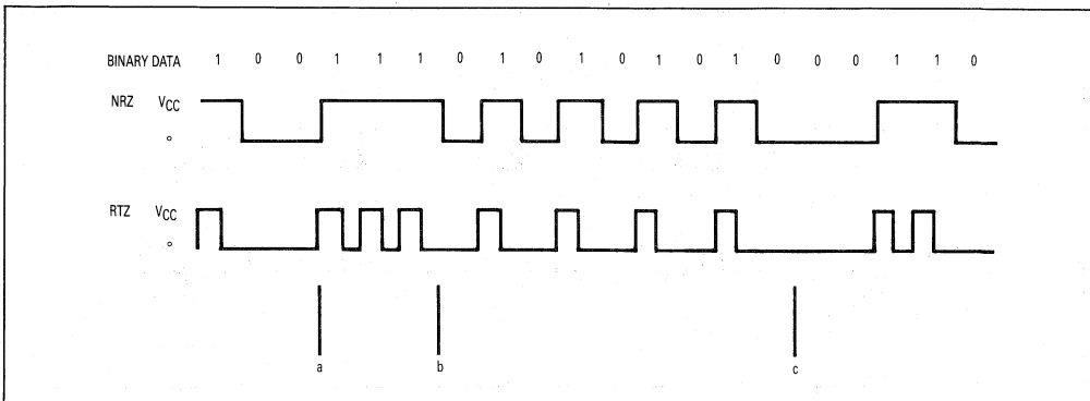
Figure 39. NRZ and RTZ Encoded Data
