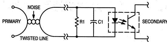
Figure 2. Noise Protection Circuits
