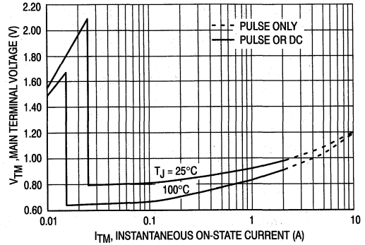
Figure 6. On-State Voltage Drop versus Output Terminal Current
