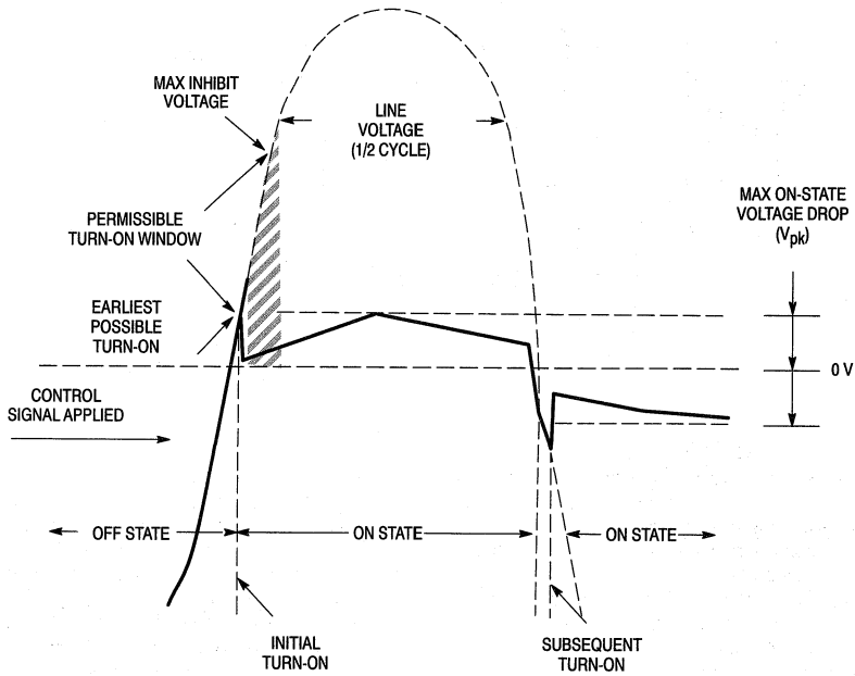
Figure 4. Zero-Voltage Turn-On Voltage Characteristics
