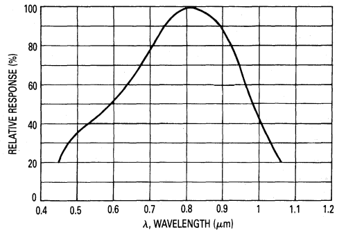
Figure 4. Constant Energy Spectral Response
