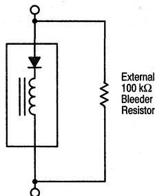
Figure 9. AC-DC Solenoid with Integral Diode
