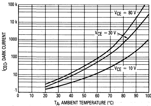
Figure 5. Collector-Emitter Dark Current versus Temperature
