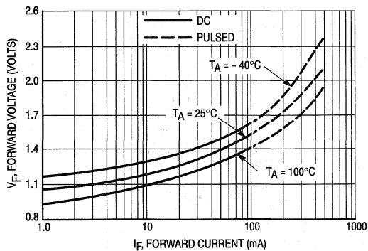
Figure 2. LED Forward Voltage versus Forward Current
