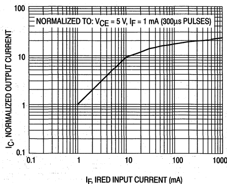
Figure 2. Output Current versus Input Current
