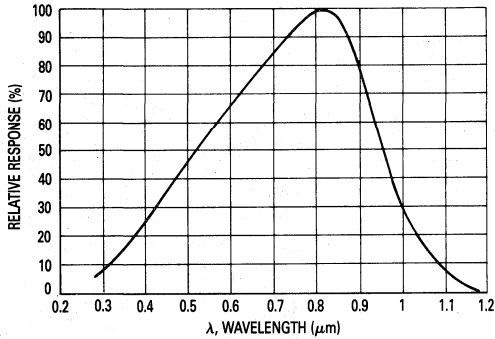
Figure 3. Relative Spectral Response
