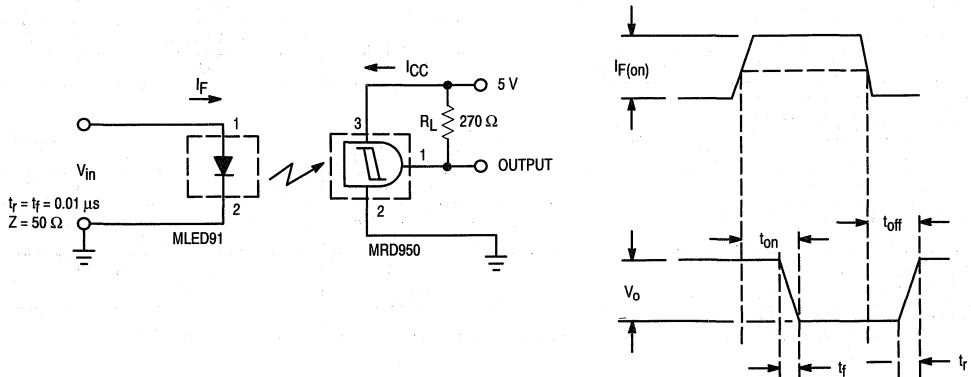
Figure 2. Switching Test Circuit
