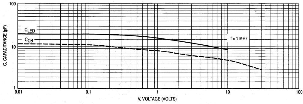
Figure 7. Capacitance versus Voltage
