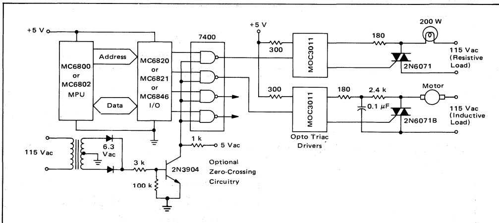
FIGURE 11 - Interfacing an M6800 Microcomputer System to 115 Vac Loads
