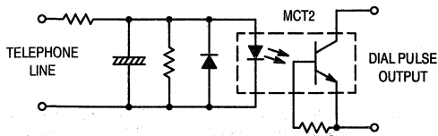
Figure 6. Dial Pulse Monitor Circuit
