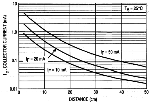
Figure 6. Current Transfer with Devices Optically Coupled
