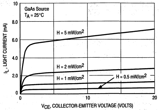
Figure 4. Transistor Collector Current versus Collector-Emitter Voltage
