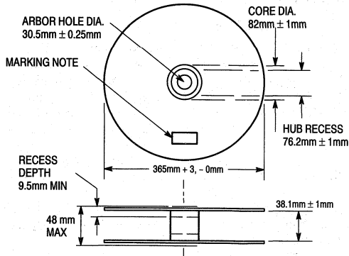
Figure 2. Reel Specifications
