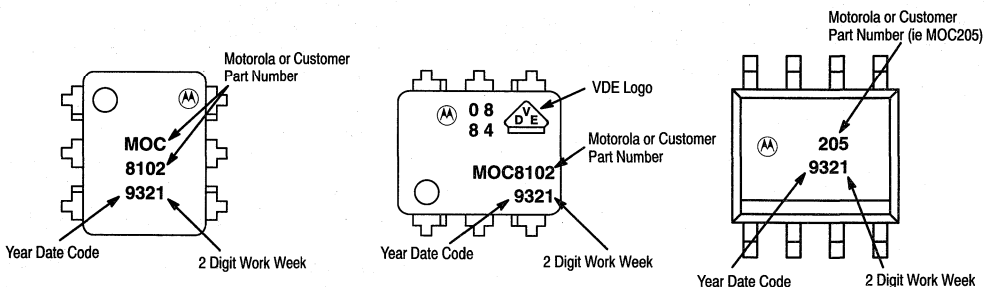
Standard 6-PIN Optoisolator Marking
