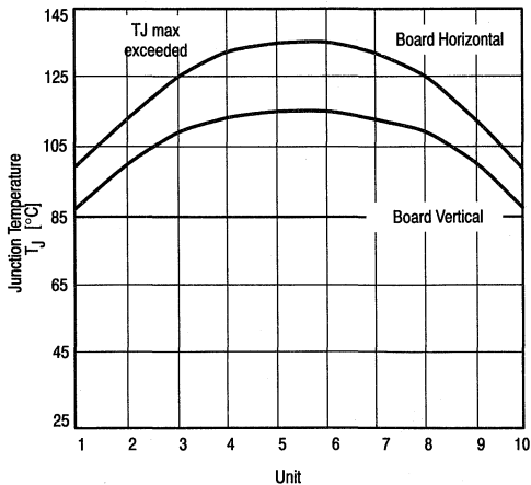
Figure 14. Cluster T J Junction Temperature Distribution in a Cluster of 10 T A = 25°C, All Devices on with I = 1 Arms
