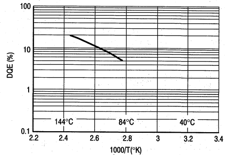
Figure 7. DQE Degradation (%)
