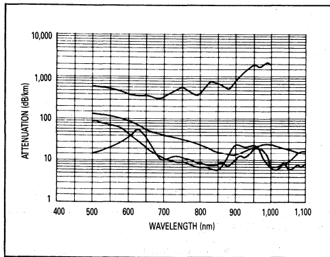
Figure 13. Fiber Attenuation versus Wavelength
