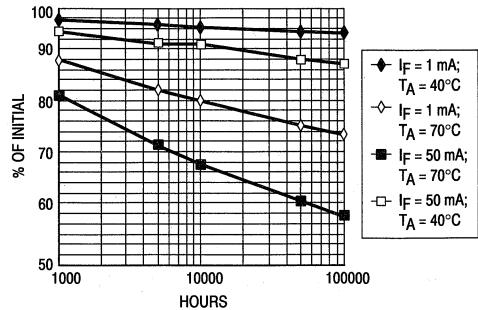
Figure 10. Six Sigma Degradation
