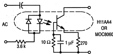
Figure 2. Ring Detector
