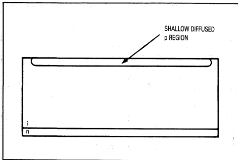
Figure 31. PIN Diode Structure
