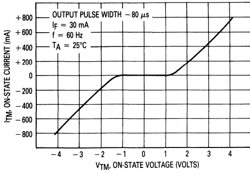
Figure 1. On-State Characteristics
