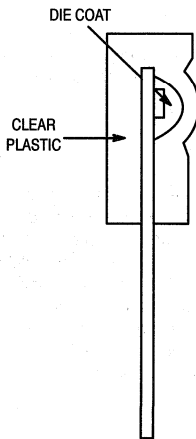
Figure 3. Case 422A Clear Epoxy Package
