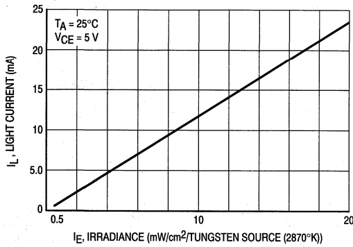
Figure 3. Collector Current versus Irradiance
