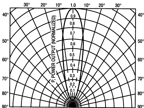
6. Divergence angle of a LED output is read directly from its radiation pattern, which is usually a part of manufacturers' data.
