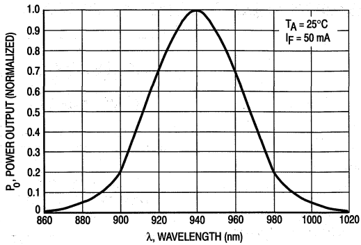
Figure 3. LED Relative Power Output versus Wavelength
