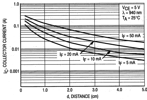
Figure 5. Collector Current versus Distance when Coupled with a Typical MLED91
