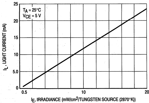
Figure 5. Transistor Collector Current versus Irradiance
