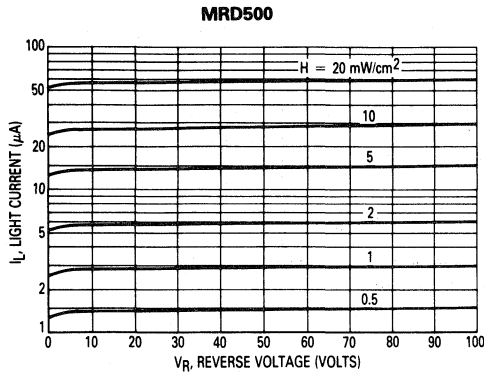
Figure 1. Irradiated Voltage — Current Characteristic
