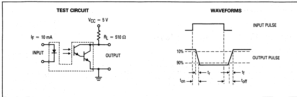
Figure 9. Switching Times
