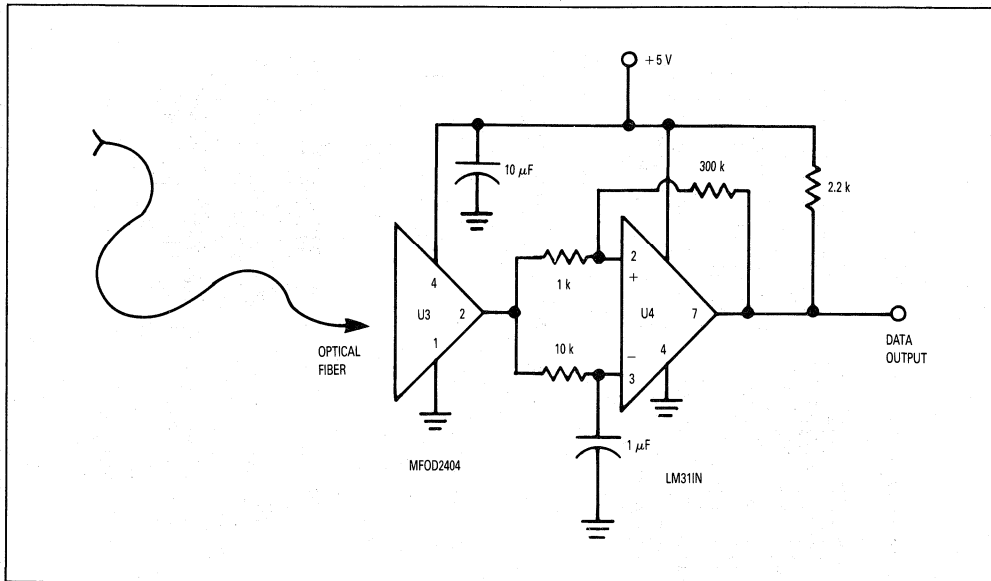
Figure 35. Simple F/O Data Receiver Using IDP And A Voltage Comparator
