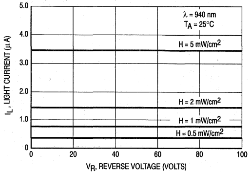
Figure 2. Light Current versus Reverse Voltage
