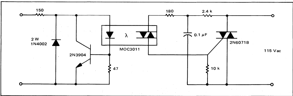
FIGURE 10 - Solid-State Relay
