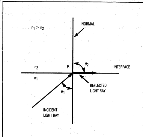
Figure 4. Critical Angle Reflection
