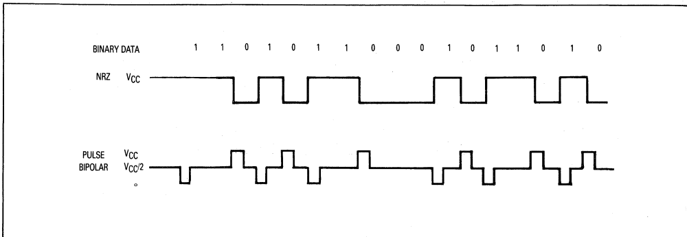
Figure 41. Pulse Bipolar Encoding
