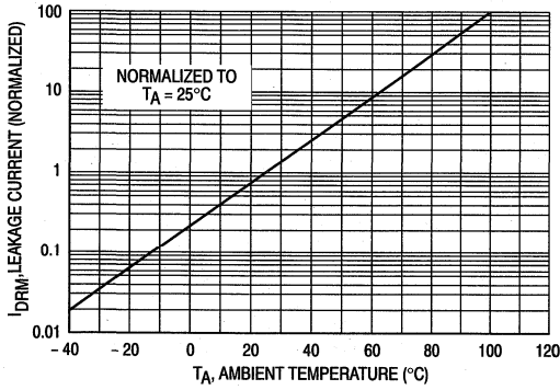
Figure 9. Leakage With LED Off versus Ambient Temperature
