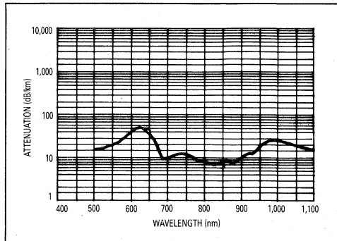
Figure 19. Attenuation versus Wavelength For A Sample Fiber
