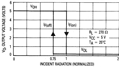
Figure 2. Transfer Characteristics
