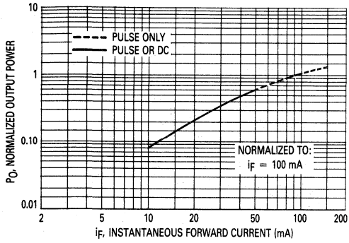
Figure 1. Normalized Output Power versus Forward Current
