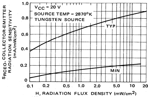
FIGURE 5 — Radiation Sensitivity for MRD901
