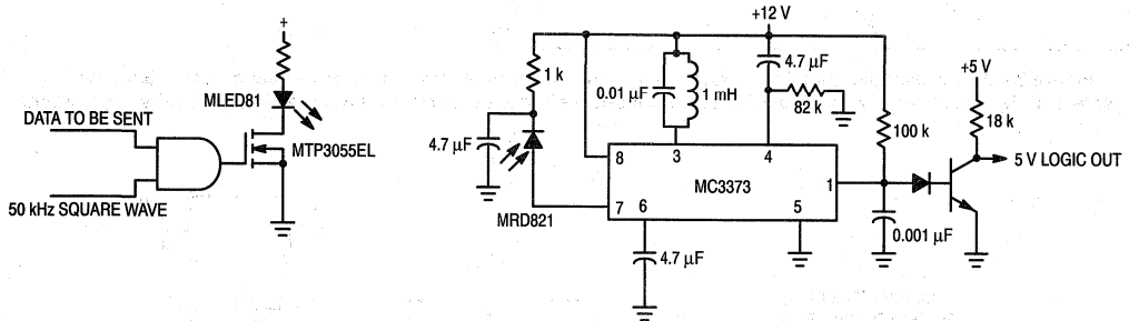
IR Receiver Using the Integrated MC3373, for Ranges of 10–30 Meters
