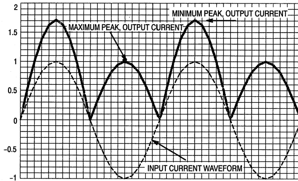
Figure 5. Output Characteristics
