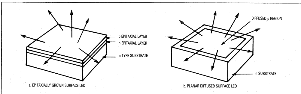
Figure 20. Simple LED Structures
