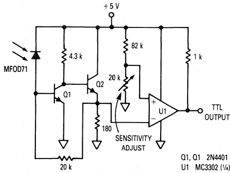
Figure 7. TTL Receiver
