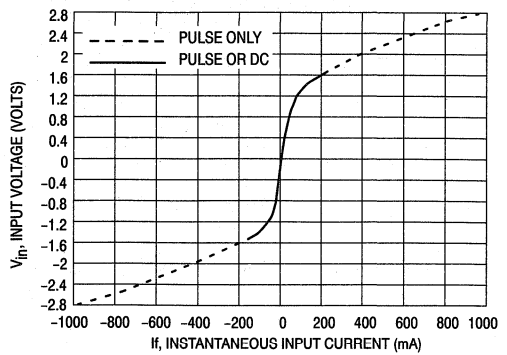
Figure 7. Input Voltage versus Input Current
