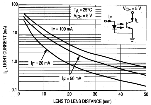
Figure 4. Coupled Characteristics of MLED91 and MRD901
