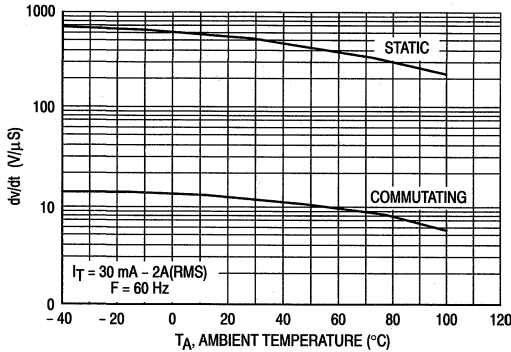
Figure 11. dv/dt versus Ambient Temperature
