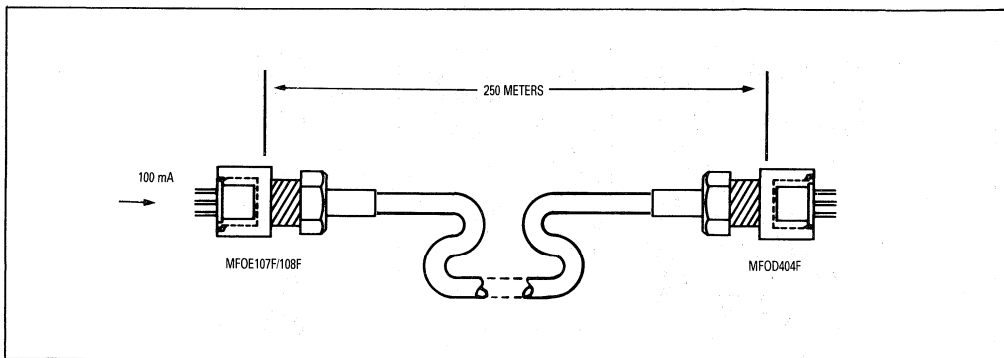
Figure 38. Simplex Fiber Optic Point To Point Link
