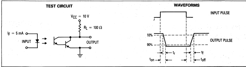
Figure 9. Switching Times
