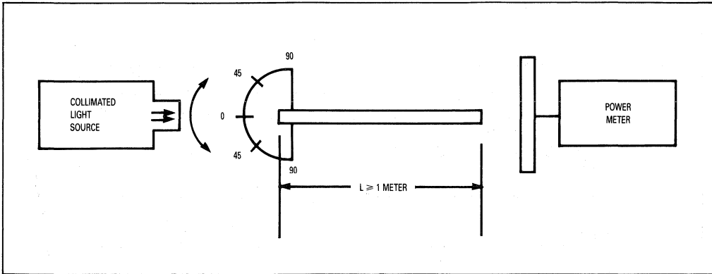
Figure 11. Measurement Of Fiber Numerical Aperture
