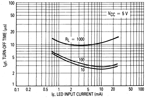
Figure 8. Turn-Off Switching Times CNY17-1 and CNY17-2
