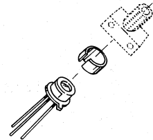
CASE 210A-01 METAL STYLE 1
