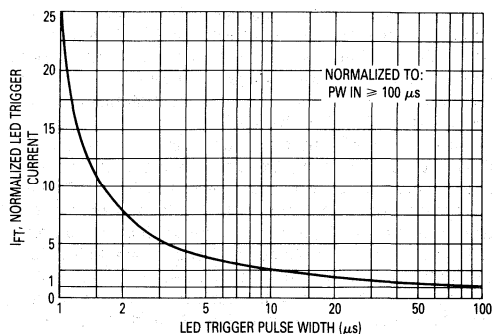
Figure 10. I_{FT} Normalized to I_{FT\text{ dc}} As Specified on the Data Sheet
