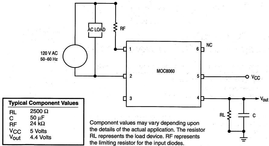
Figure 8. Typical Application Circuit: AC to DC Detector Circuit
