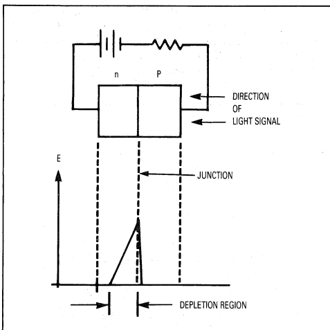
Figure 29. Electric Field In A Reverse-Biased PN Photodiode
