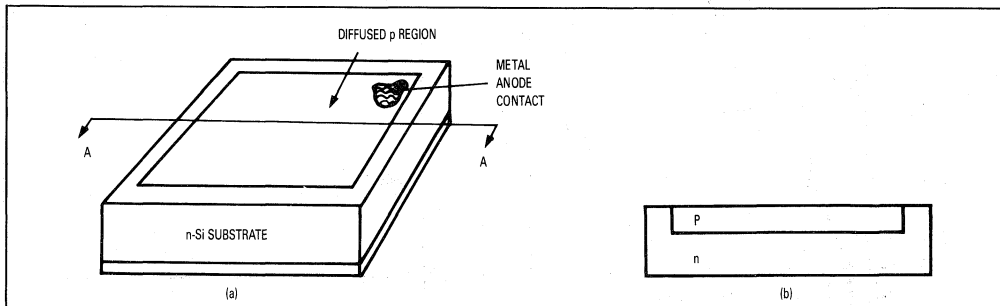
Figure 27. PN Photodiode: (a) Device (b) Section View at AA
