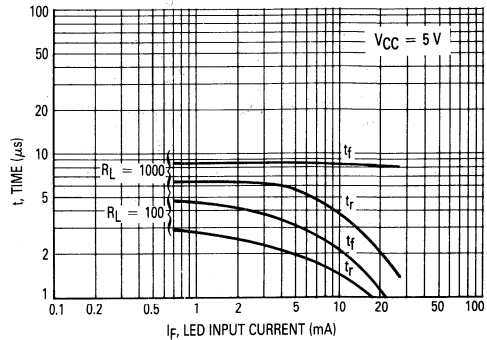
Figure 6. Rise and Fall Times CNY17-1 and CNY17-2
