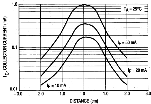
Figure 7. Translational Optical Coupling at 5 mm Separation (Lens to Lens)
