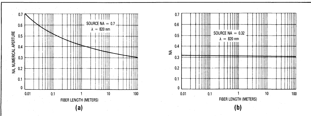
Figure 12. Fiber Numerical Aperture versus Length For Two Values Of Source N.A.
