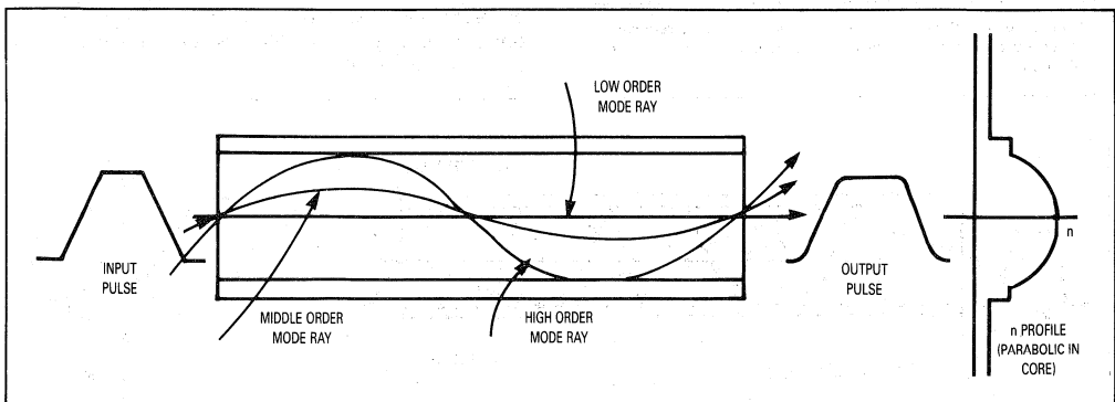
Figure 16. Propagation Along A Multimode Graded Index Fiber
