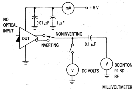
Test Circuit A
