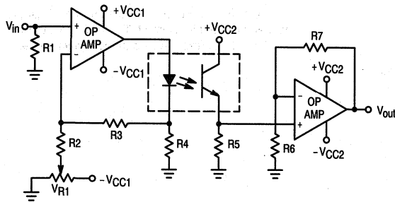
Figure 1. Isolation Amplifier
