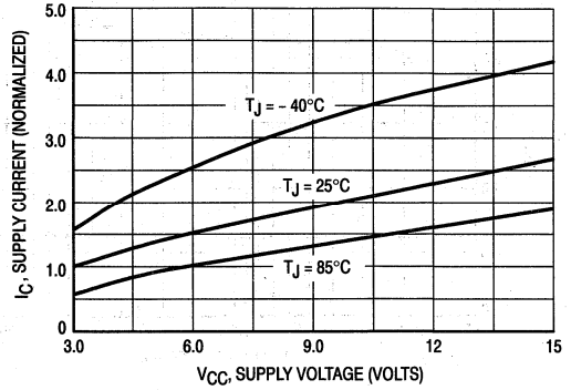
Figure 4. Supply Current versus Supply Voltage — Output High
