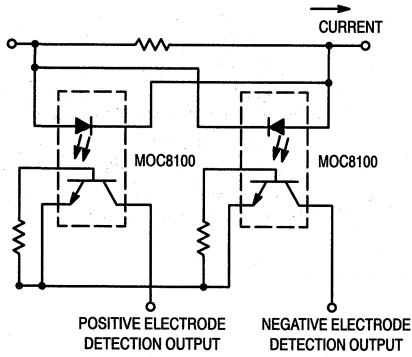
Figure 7. Telephone Line Polarity Detection Circuit
