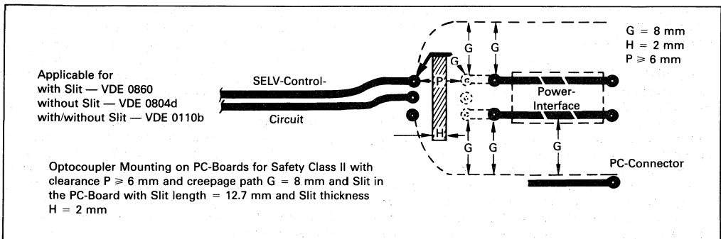
Figure 4. Optocoupler Mounting on PC Boards for Safety Class II with Clearance
