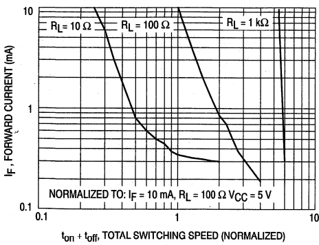
Figure 6. Input Current versus Total Switching Speed
