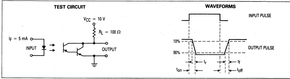
Figure 9. Switching Times
