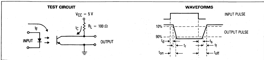
Figure 11. Switching Times
