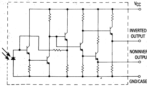
Figure 1. Equivalent Schematic
