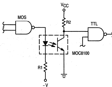
Figure 5. Level Conversion Circuit
