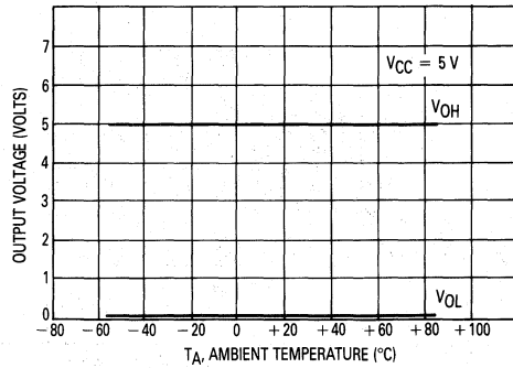
Figure 7. Output Voltage versus Ambient Temperature
