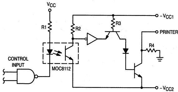
Figure 8. Print Head Circuit Control
