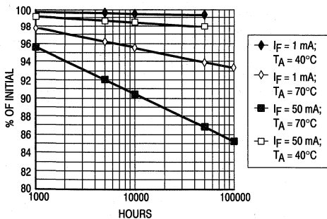
Figure 9. Average Degradation
