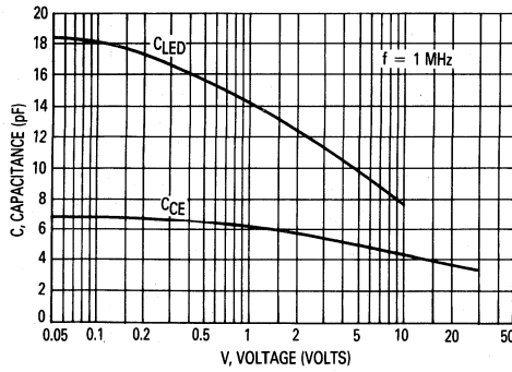
Figure 9. Capacitances versus Voltage
