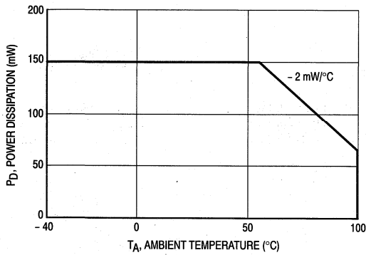
Figure 1. Power Dissipation
