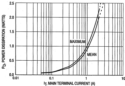
Figure 7. Power Dissipation versus Main Terminal Current
