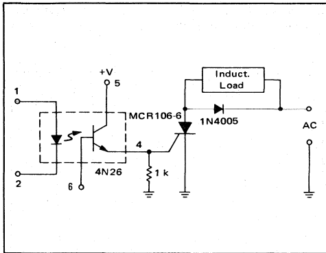
FIGURE 11 – Coupler-Driven SCR
