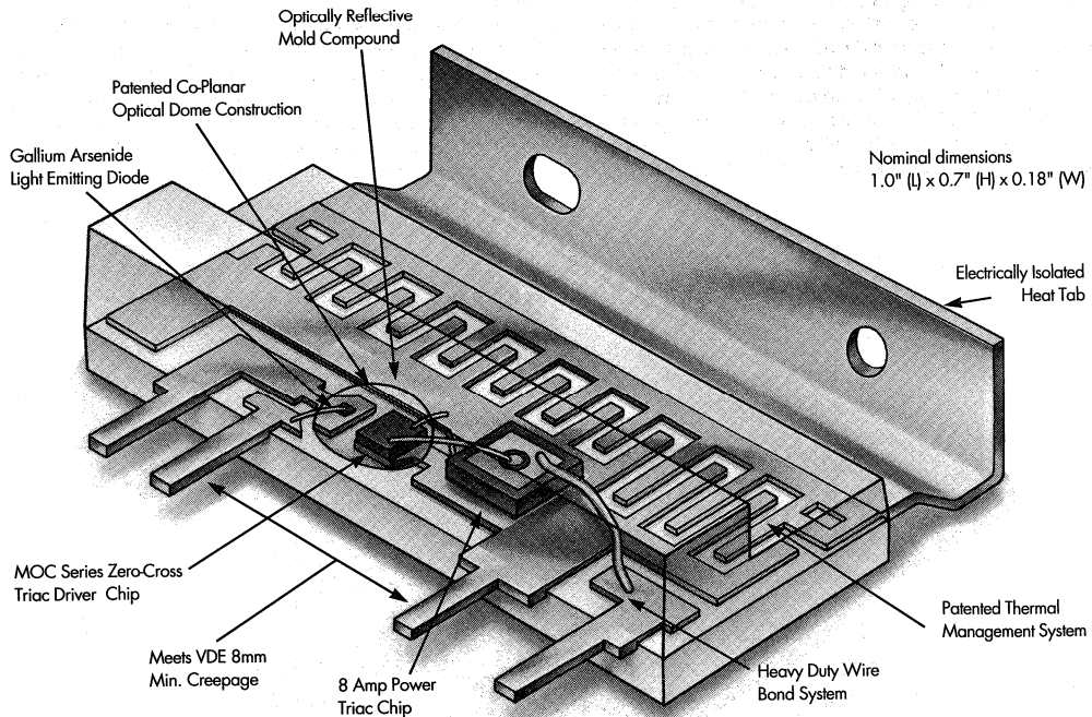
Figure 1. Internal Construction of the POWER OPTO Isolator
