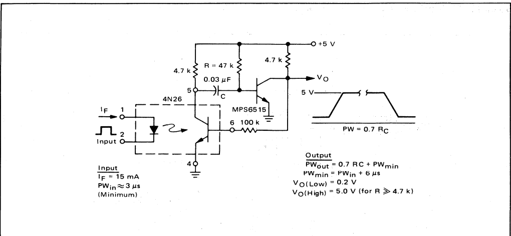
FIGURE 15 — Pulse Stretcher
