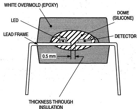
Figure 2. Geometric Design for Optoisolators
