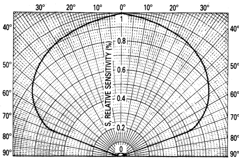
Figure 3. Angular Response
