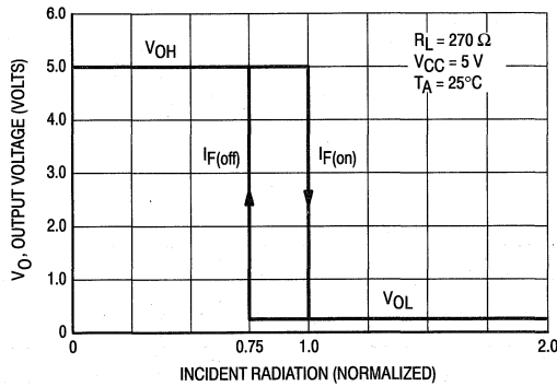
Figure 1. Transfer Characteristics
