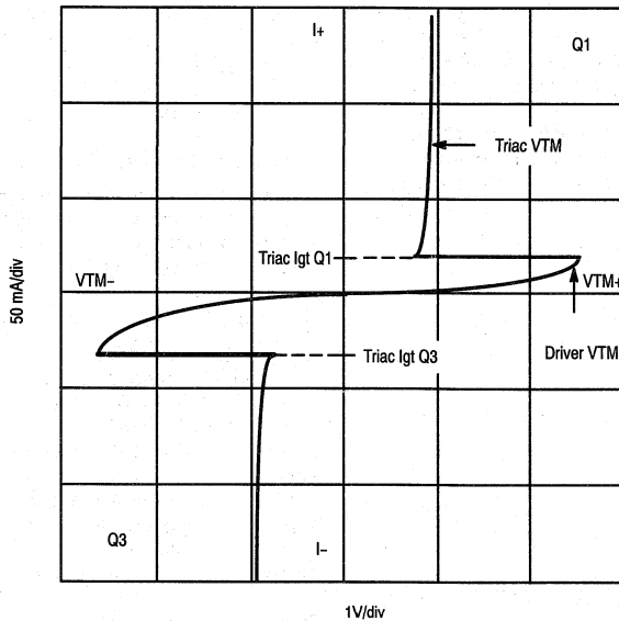
Figure 5. Curve Tracer Voltage versus Current Plot
