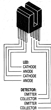
CASE 792-01 STYLE 2
