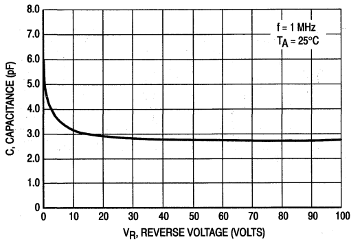
Figure 5. Capacitance versus Voltage
