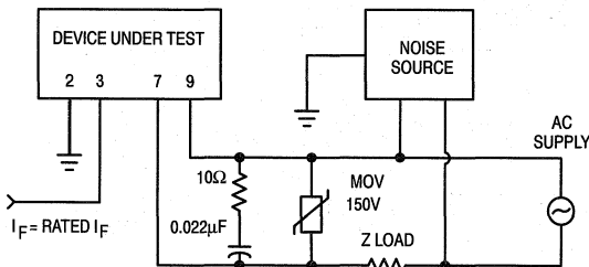
Figure 15. Test Circuit for Conducted Noise Tests
