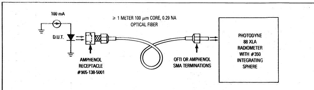
Figure 4. Launched Power (P L ) Test Set
