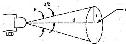
4. Area irradiated by a light-emitting diode (LED) can be computed from this sketch.
