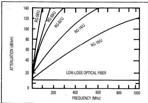
Figure 18. Comparative Attenuation versus Frequency For Optical Fiber and Coax Cable
