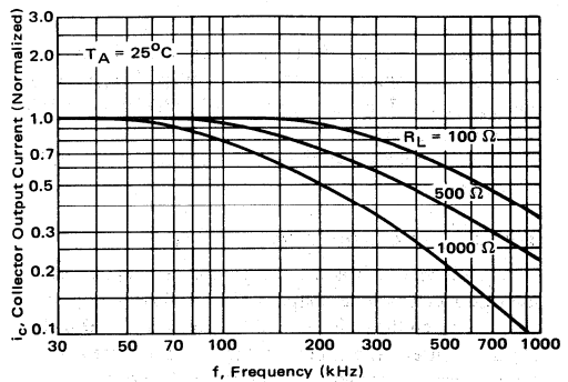
FIGURE 6 – Frequency Response
