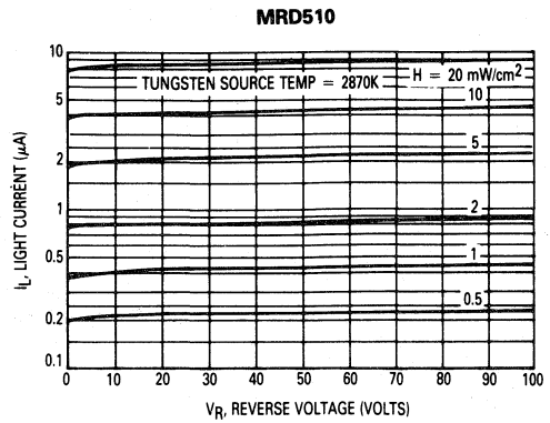
Figure 1. Irradiated Voltage — Current Characteristic
