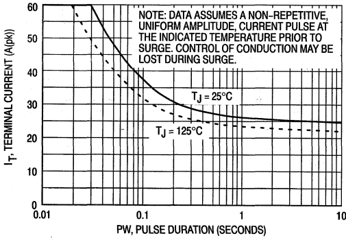
Figure 5. Maximum Allowable Surge Current versus Pulse Duration
