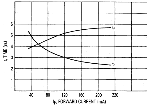
Figure 12. Rise and Fall Time versus Forward Current
