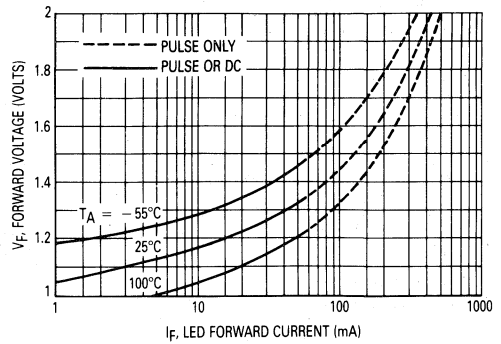
Figure 4. Forward Characteristics
