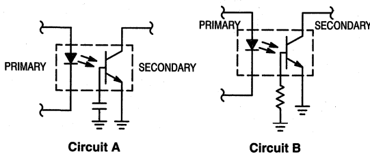
Figure 3. Noise Protection Circuits
