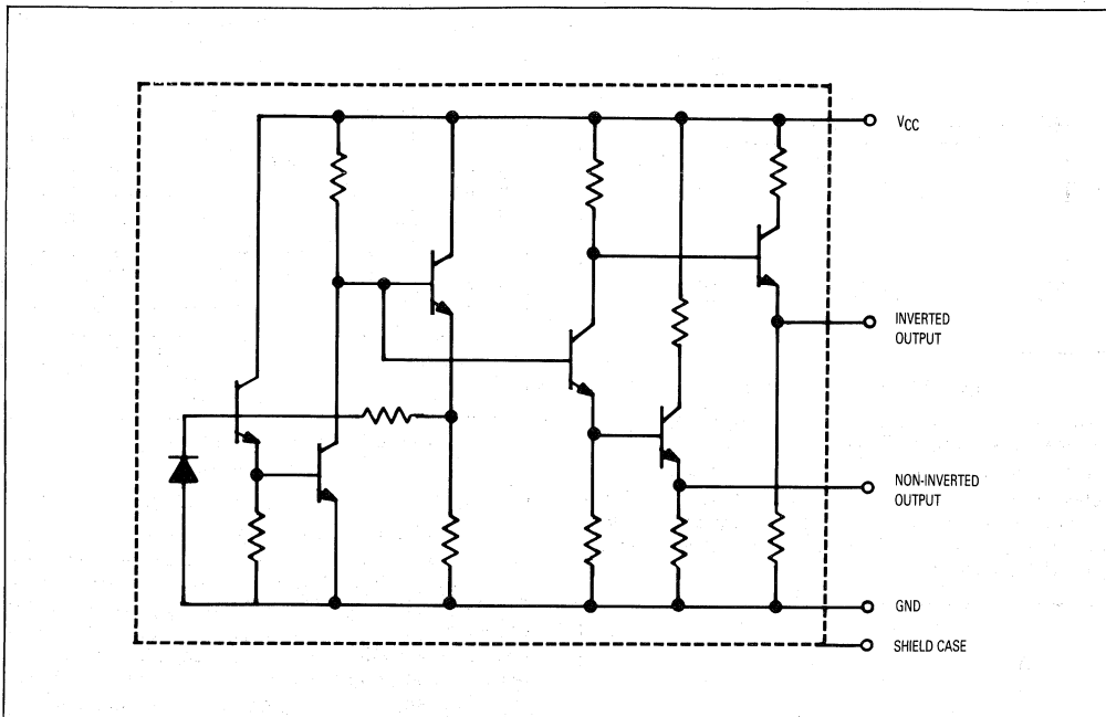
Figure 34. Integrated Detector Preamplifier
