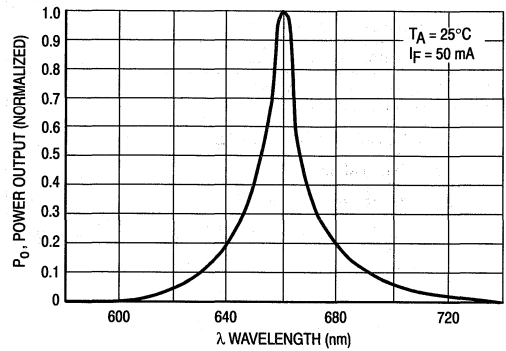
Figure 4. Relative Spectral Emission
