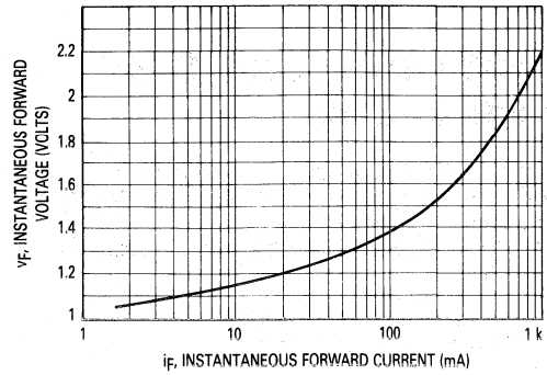
Figure 2. Forward Characteristics
