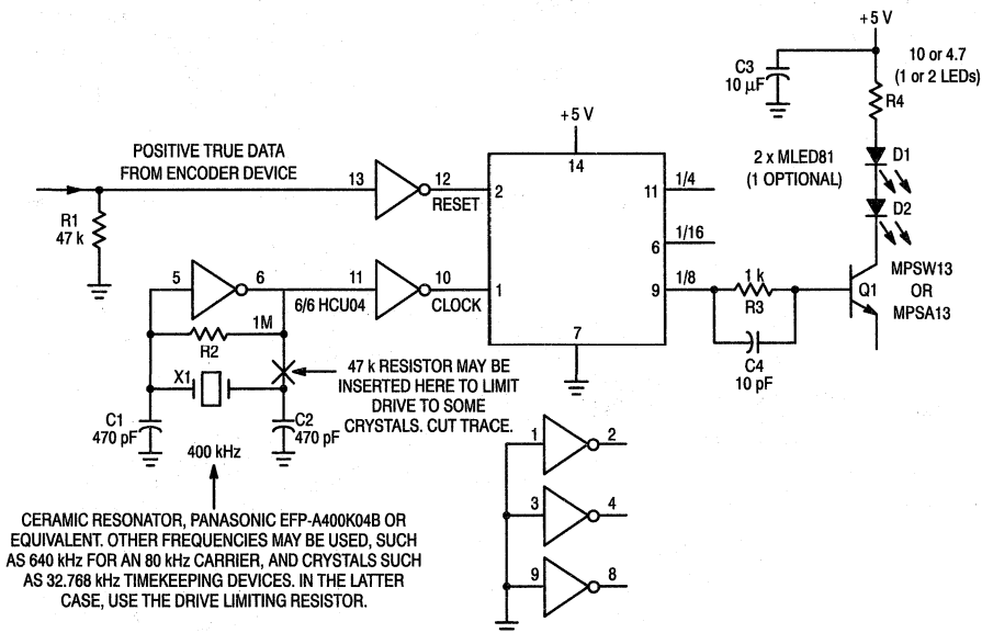
Figure 3b. IR Transmitter section: Note that the use of two IR LEDs is optional. Choose R4 for an LED current appropriate to the application. 250 mA is typical.
