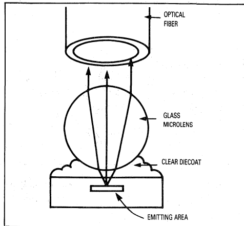
Figure 23. Increasing Light Coupling With A Microsphere
