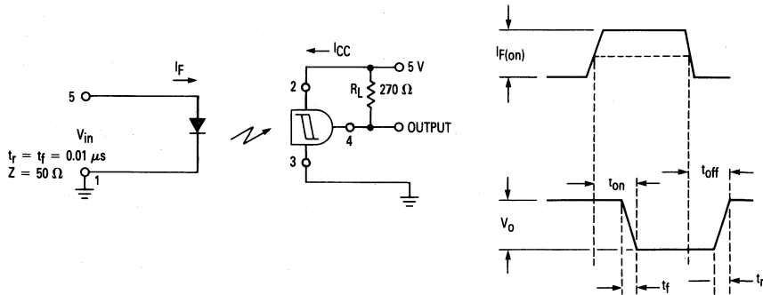
Figure 9. Switching Test Circuit
