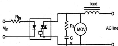
Figure 6. Application with Snubber and MOV
