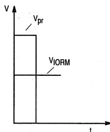
Test voltage curve (ac) for routine tests.
