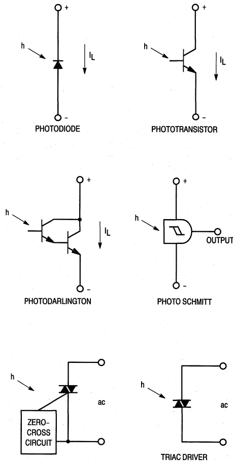
Figure 3. Light Sensitive Detectors
