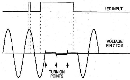
Figure 12. Operating Waveforms
