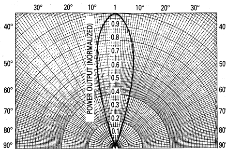
Figure 5. Spatial Radiation Pattern
