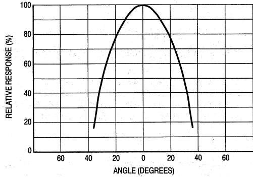
Figure 2. Angular Response
