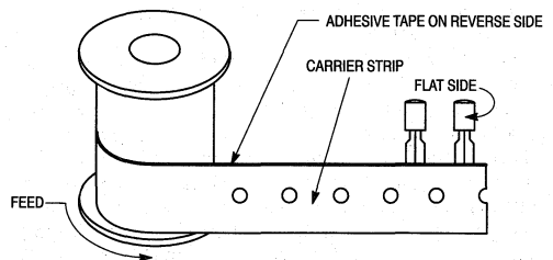
Figure 2. Reel Specifications
