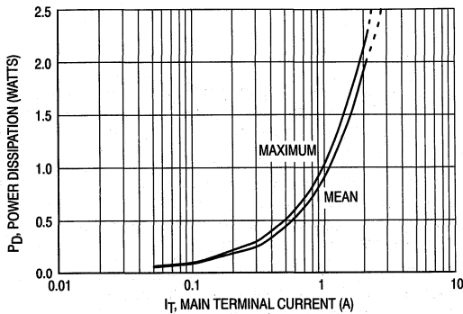
Figure 7. Power Dissipation versus Main Terminal Current
