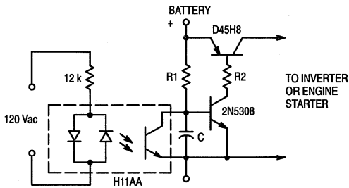
Figure 3. UPS Solid State Turn-On Switch
