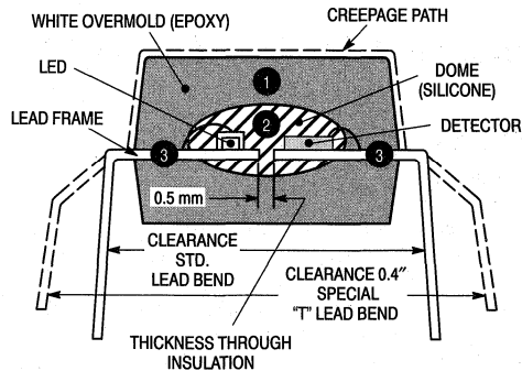
Figure 2. Coplanar Die Placement
