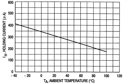
Figure 10. Holding Current versus Ambient Temperature
