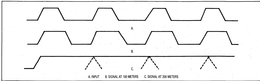
Figure 15. Loss Of Pulse Identity Due To Pulse Width Dispersion
