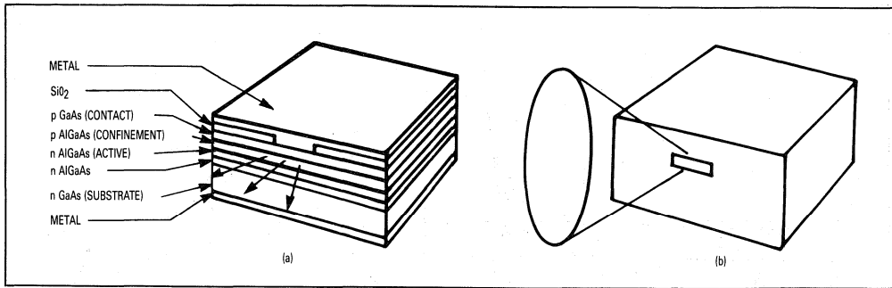
Figure 26. Edge Emitting LED: (a) Structure (b) Beam Pattern
