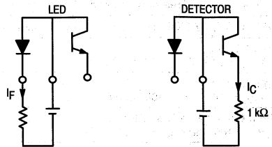
Figure 8. Test Circuit for Figures 6 and 7
