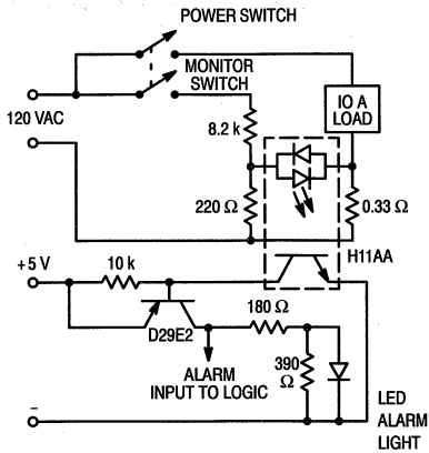
Figure 1. Load Monitor and Alarm
