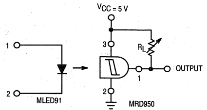
Figure 12. Test Circuit for Output Voltage versus Load Current Measurements
