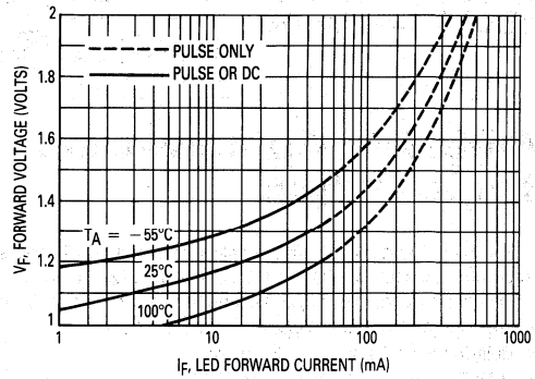
Figure 4. LED Forward Characteristics
