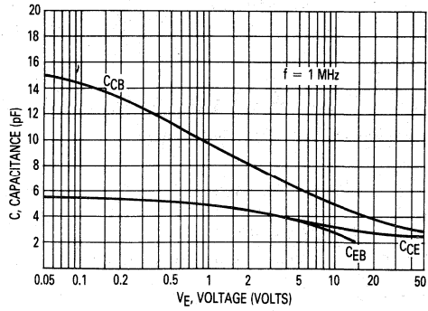
Figure 10. Detector Capacitances versus Voltage
