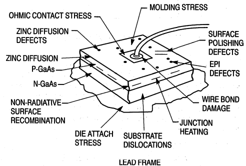
Figure 2. LED Degradation Sources
