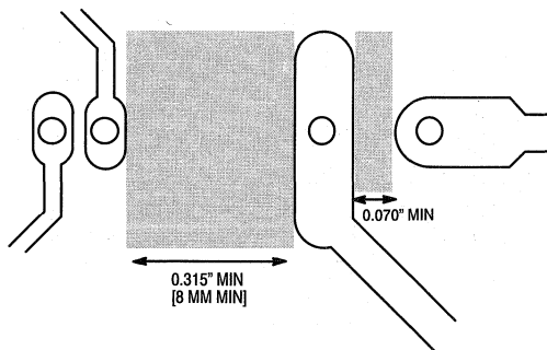
Figure 14. PC Board Layout Recommendations
