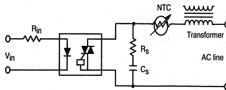
Figure 8. Thermistor Limits Excessive Inrush Current
