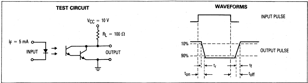
Figure 9. Switching Times
