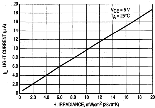
Figure 7. Light Current versus Irradiance
