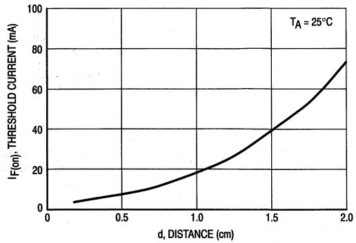
Figure 8. Threshold Current versus Lens Separation Distance at 25°C
