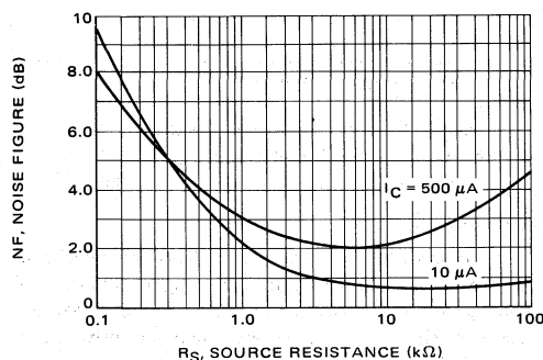
FIGURE 18 — MRD300 Noise Figure versus Source Resistance
