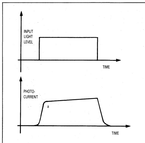
Figure 30. Pulse Response Of A Photodiode
