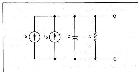
FIGURE 5 – Approximate Model of Photodiode
