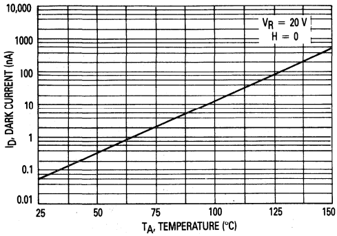
Figure 1. Dark Current versus Temperature
