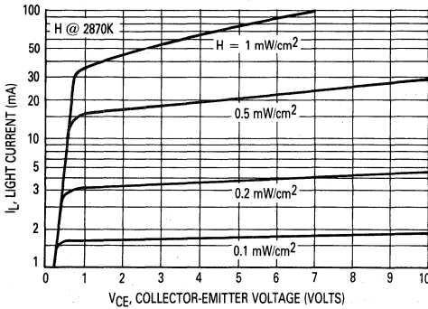
Figure 3. Collector Characteristics
