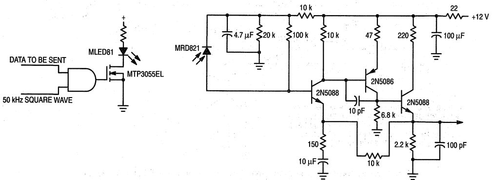
High-Performance Discrete Front-End Amplifier with Special Attention Paid to Noise for Range of up to 100 Meters
