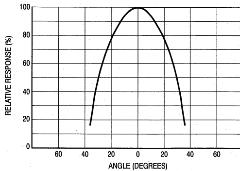
Figure 5. Angular Response
