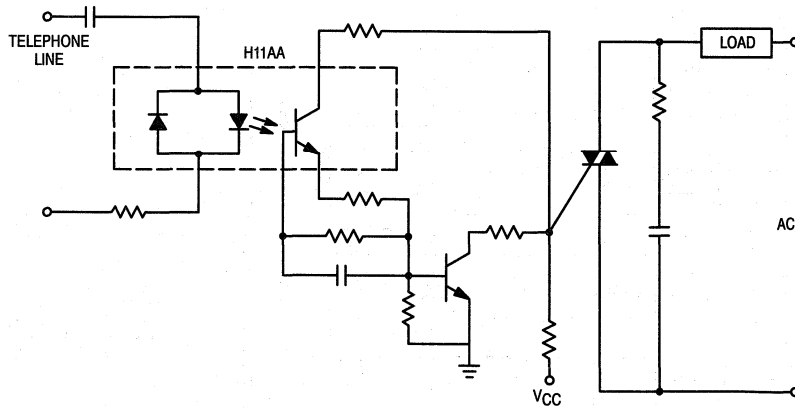
Figure 4. Power Control by Bell Signal Circuit
