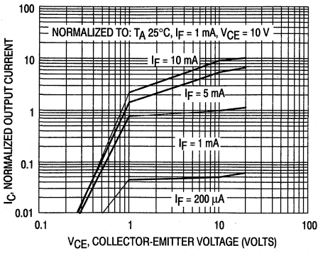
Figure 3. Output Current versus Collector-Emitter Voltage
