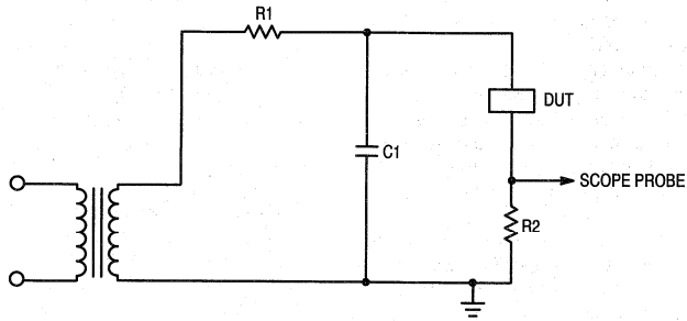
Figure 2. Wideband Partial Discharge Test Circuit
