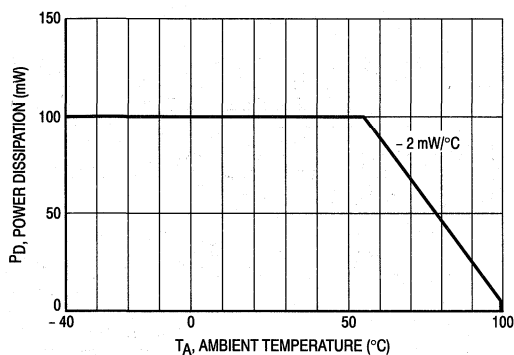
Figure 1. Power Dissipation
