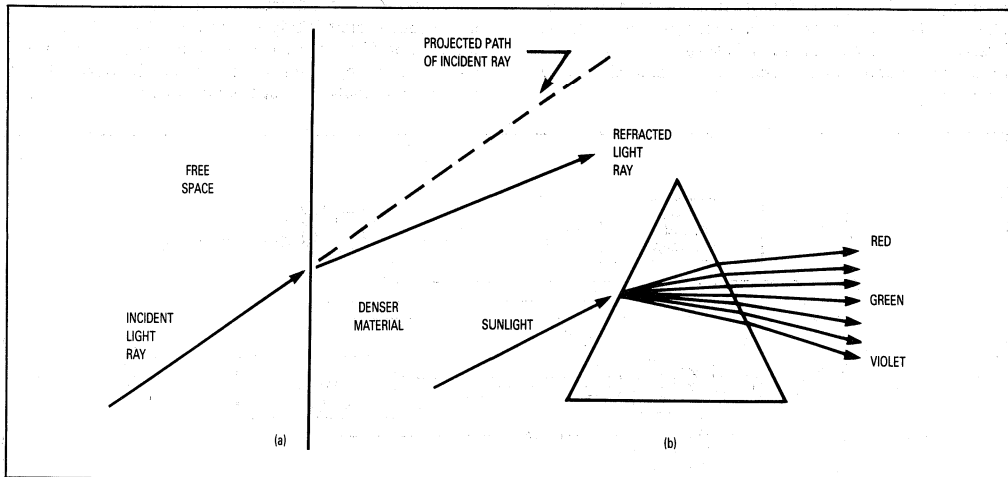
Figure 2. Refraction Of Light:
