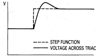
Figure 14. Voltage Waveform After Step Voltage Rise — Resonant Snubbing
