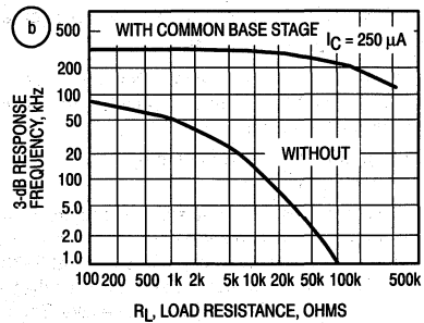
8. Improved frequency response of a phototransistor is obtained with a common-base load-impedance transforming network (a) in either the collector or emitter circuit. The degree of the improvement is shown in "b".
