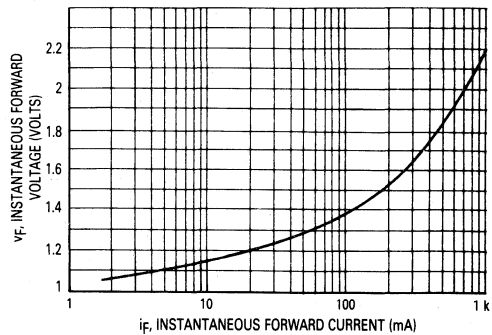
Figure 8. MLED930 Forward Characteristics
