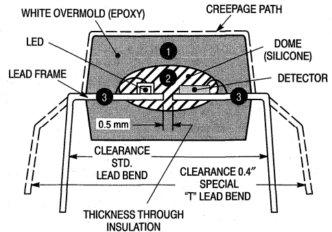
Figure 3. "DOME" Package
