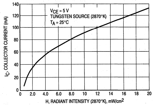
Figure 4. Collector Current versus Radiant Intensity
