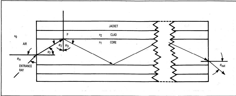
Figure 8. Ray Propagation In A Fiber
