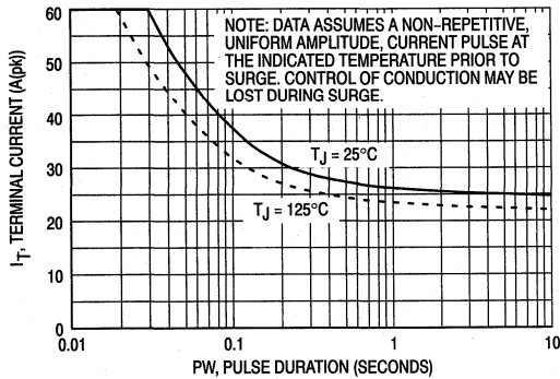
Figure 5. Maximum Allowable Surge Current versus Pulse Duration
