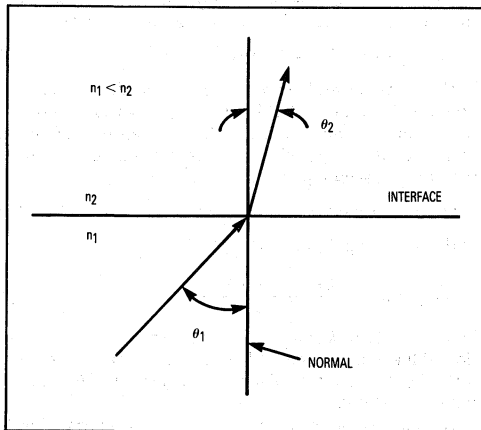
Figure 3. Refractive Model For Snell's Law
