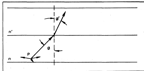
FIGURE 15 – Ray Refraction at an Interface
