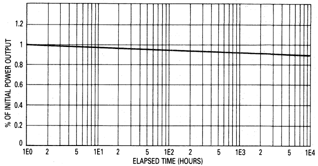
Figure 4. Power Output versus Time
