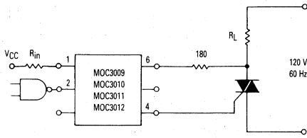
Figure 8. Resistive Load
