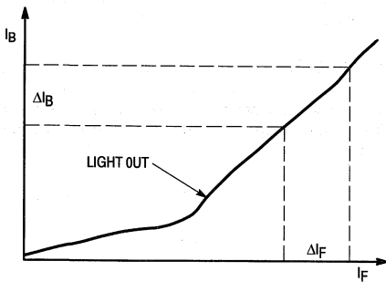
Figure 6. DQE is Expressed as \Delta I_B Divided by \Delta I_F
