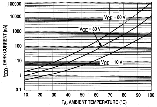
Figure 4. Collector-Emitter Dark Current versus Temperature
