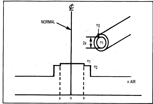
Figure 7. Index Profile For A Step Index Fiber
