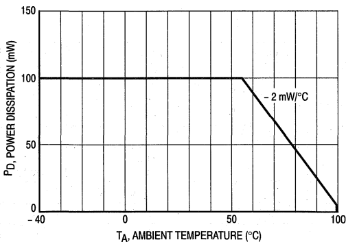
Figure 1. Power Dissipation
