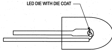
Figure 4. Panel Mount LED
