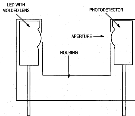
Figure 1. Typical Slotted Interrupter
