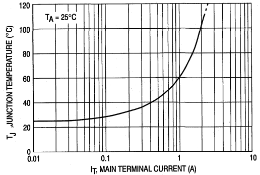
Figure 8. Junction Temperature versus Main Terminal RMS Current (Free Air)
