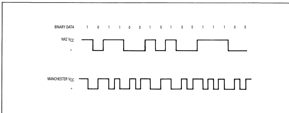
Figure 40. Manchester Data Encoding
