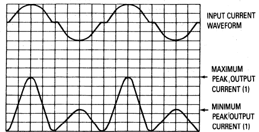
Figure 2. Output Characteristics
