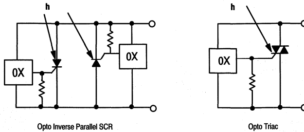
Figure 3. Triac Driver Simplified Circuits
