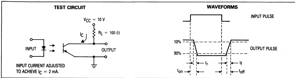
Figure 10. Switching Times
