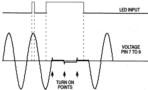
Figure 12. Operating Waveforms
