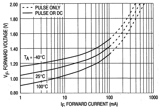
Figure 2. LED Forward Voltage versus LED Forward Current
