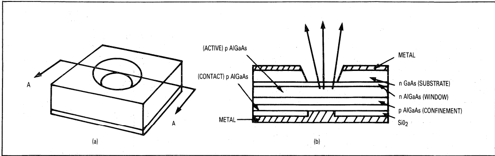
Figure 24. Burrus, Or Etched Well, LED: (a) Device (b) Crosssection at AA
