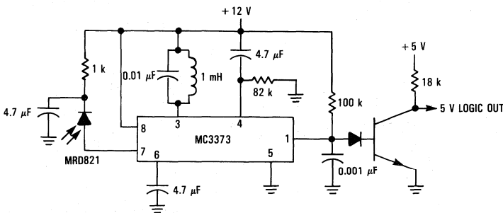
Figure 8. IR Receiver Using the Integrated MC3373
