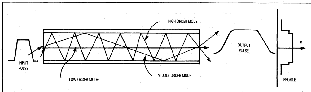
Figure 14. Propagation Along A Multimode Step Index Fiber
