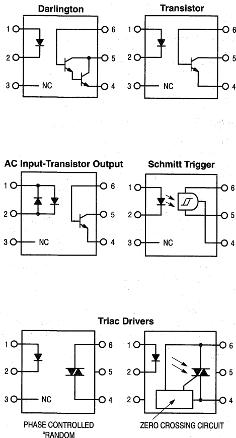
Figure 6. Various Optoisolator Configurations
