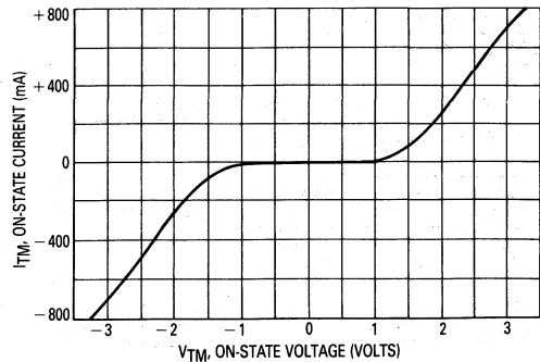
Figure 2. On-State Characteristics
