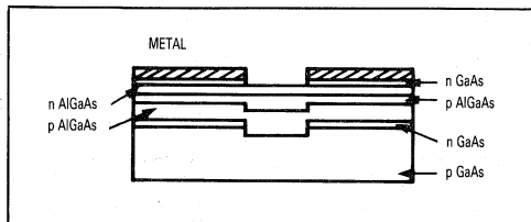
Figure 22. Section AA Of Planar Heterojunction LED
