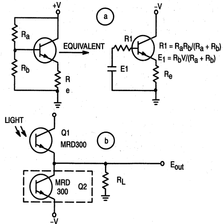
7. Temperature-compensation methods for a three-lead phototransistor are quite similar to a classical bias-stabilization approach (a). In the case of a two lead device, a matched pair of phototransistors can be used, one to receive the normal light input, while the other is masked (b).
