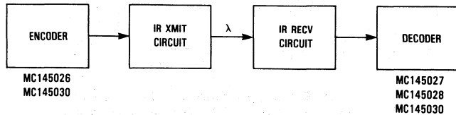
Figure 11. Utilizing Motorola's Encoders and Decoders
