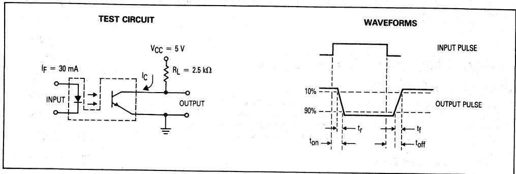
Figure 9. Switching Times
