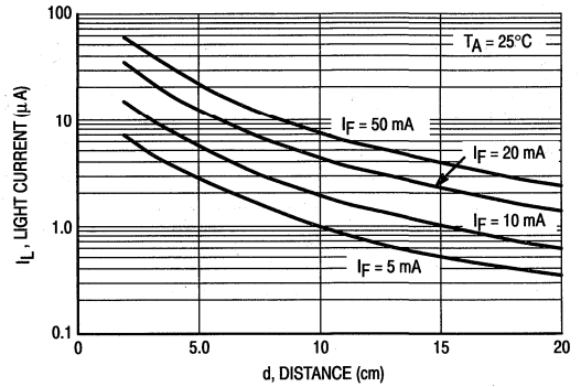
Figure 8. Light Current versus Distance when Coupled with a Typical MLED91
