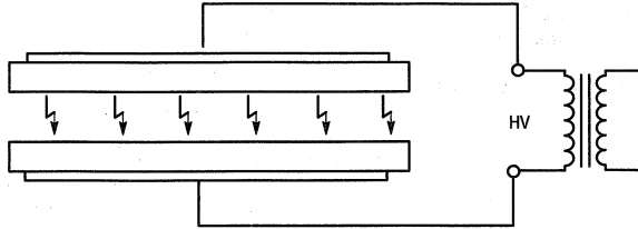
Figure 1b. Corona Discharge Between Two Glass Plates
