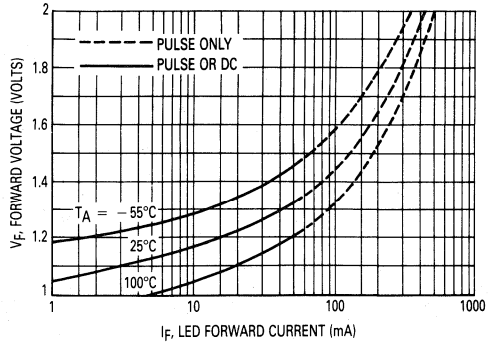
Figure 4. Forward Characteristics
