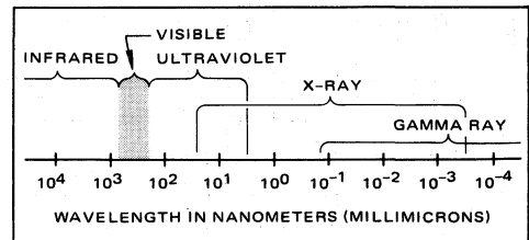
FIGURE I-1 — Portion of Electromagnetic Spectrum
