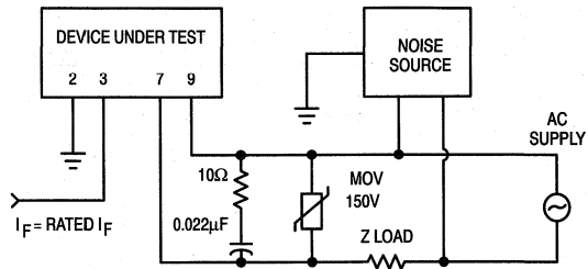
Figure 15. Test Circuit for Conducted Noise Tests
