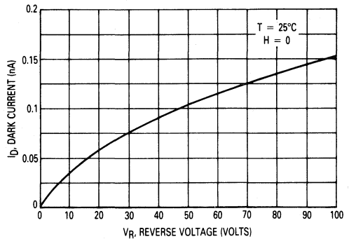
Figure 3. Dark Current versus Reverse Voltage
