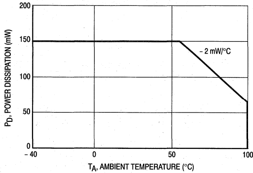
Figure 1. Power Dissipation
