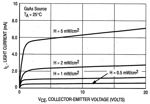
Figure 2. IC versus V CE
