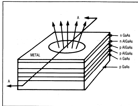
Figure 21. Planar Heterojunction LED
