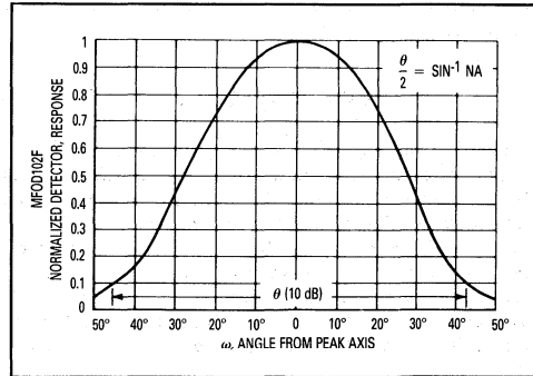
Figure 10. Graphical Definition Of Numerical Aperture
